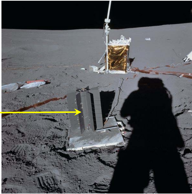
In the foreground, the radioisotope thermoelectric generator. In the background, the central post. Apollo 14 Mission . NASA Photo.
