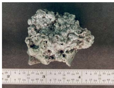
Alumina particle from a space shuttle. NASA Photo
